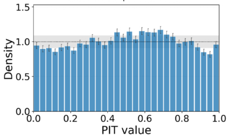
Flow-Spline CDE -2.593 | PIT-KS 0.027
