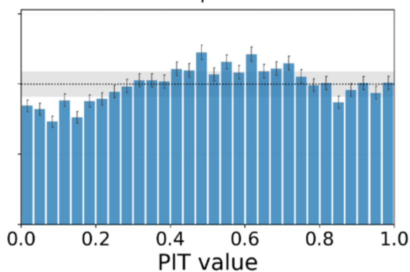
MDN (deep) CDE -2.454 | PIT-KS 0.043
