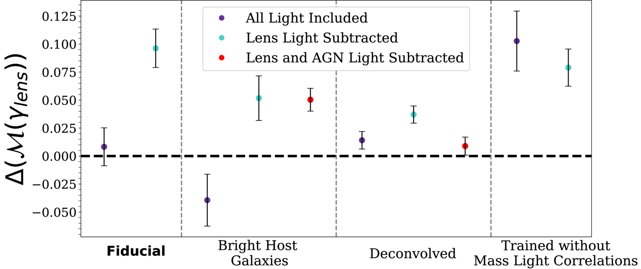
Figure 9. from Padmavathi Venkatraman et al 2026 Astron. J. 172 doi:10.3847/1538-3881/ae9e2b https://dx.doi.org/10.3847/1538-3881/ae9e2b © 2026. The Author(s). Published by the American Astronomical Society.
