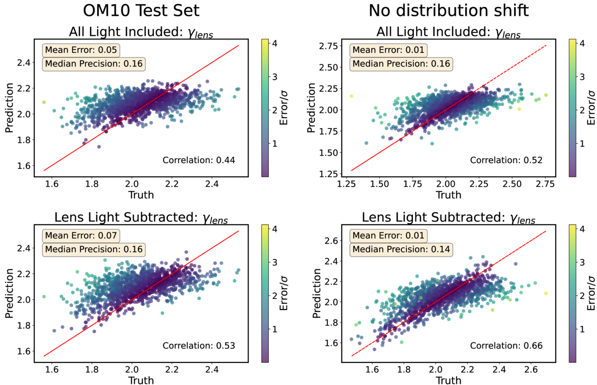
Figure 8. from Padmavathi Venkatraman et al 2026 Astron. J. 172 doi:10.3847/1538-3881/ae9e2b https://dx.doi.org/10.3847/1538-3881/ae9e2b © 2026. The Author(s). Published by the American Astronomical Society.
