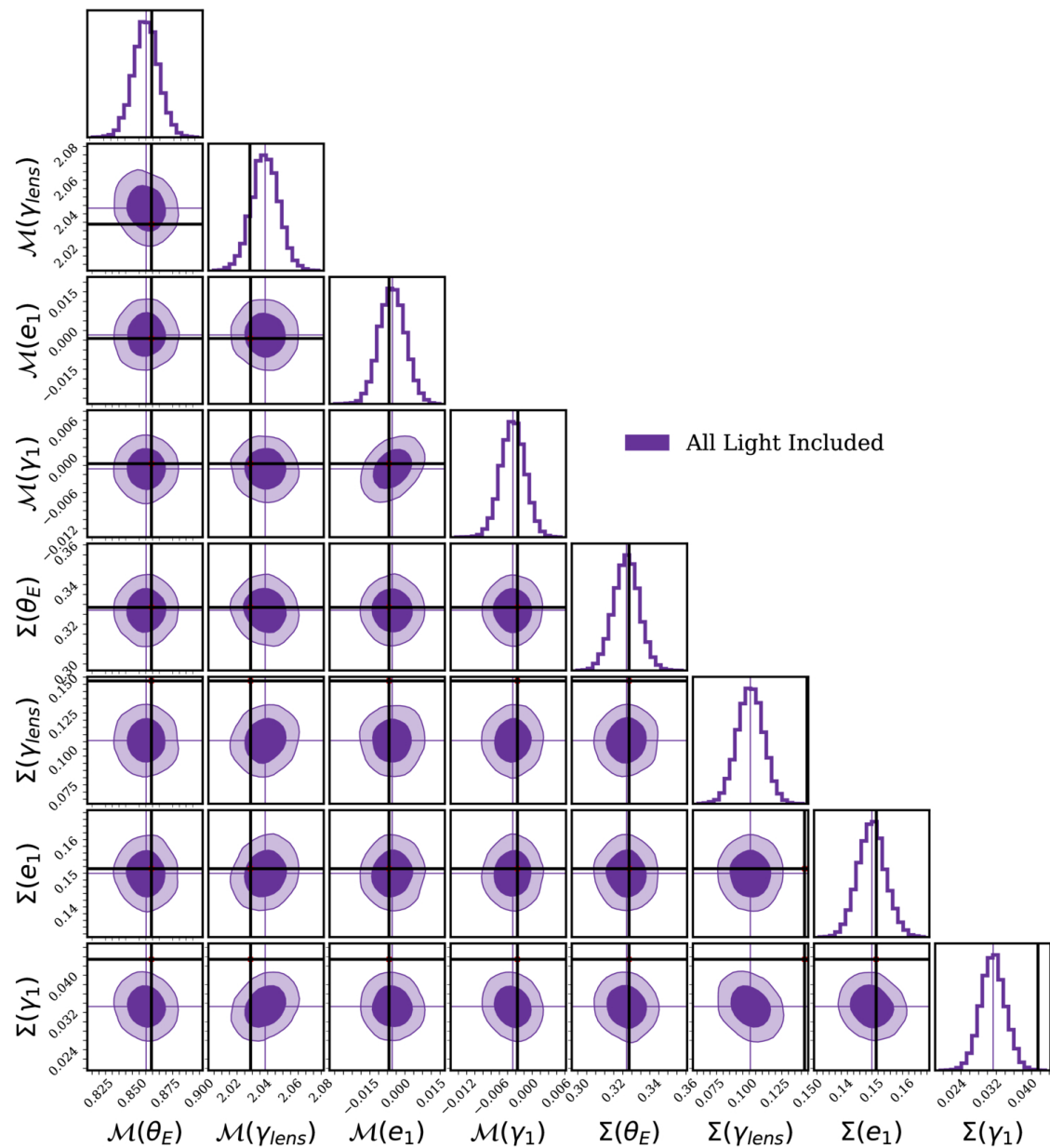
Figure 7. from Padmavathi Venkatraman et al 2026 Astron. J. 172 doi:10.3847/1538-3881/ae9e2b https://dx.doi.org/10.3847/1538-3881/ae9e2b © 2026. The Author(s). Published by the American Astronomical Society.
