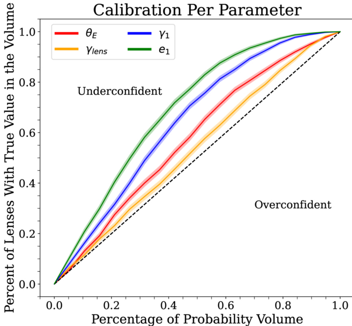
Figure 6. from Padmavathi Venkatraman et al 2026 Astron. J. 172 doi:10.3847/1538-3881/ae9e2b https://dx.doi.org/10.3847/1538-3881/ae9e2b © 2026. The Author(s). Published by the American Astronomical Society.
