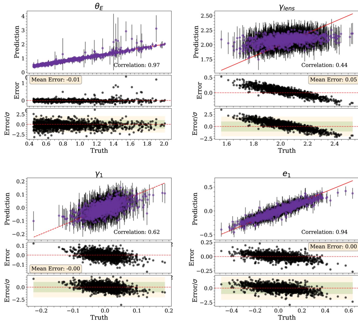
Figure 5. from Padmavathi Venkatraman et al 2026 Astron. J. 172 doi:10.3847/1538-3881/ae9e2b https://dx.doi.org/10.3847/1538-3881/ae9e2b © 2026. The Author(s). Published by the American Astronomical Society.
