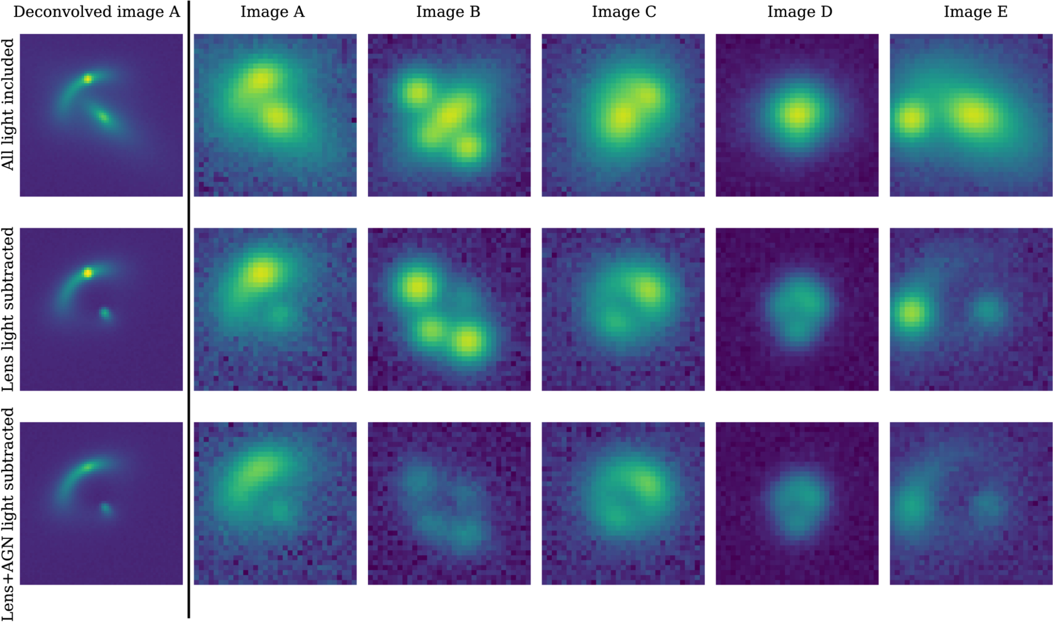
Figure 4. from Padmavathi Venkatraman et al 2026 Astron. J. 172 doi:10.3847/1538-3881/ae9e2b https://dx.doi.org/10.3847/1538-3881/ae9e2b © 2026. The Author(s). Published by the American Astronomical Society.
