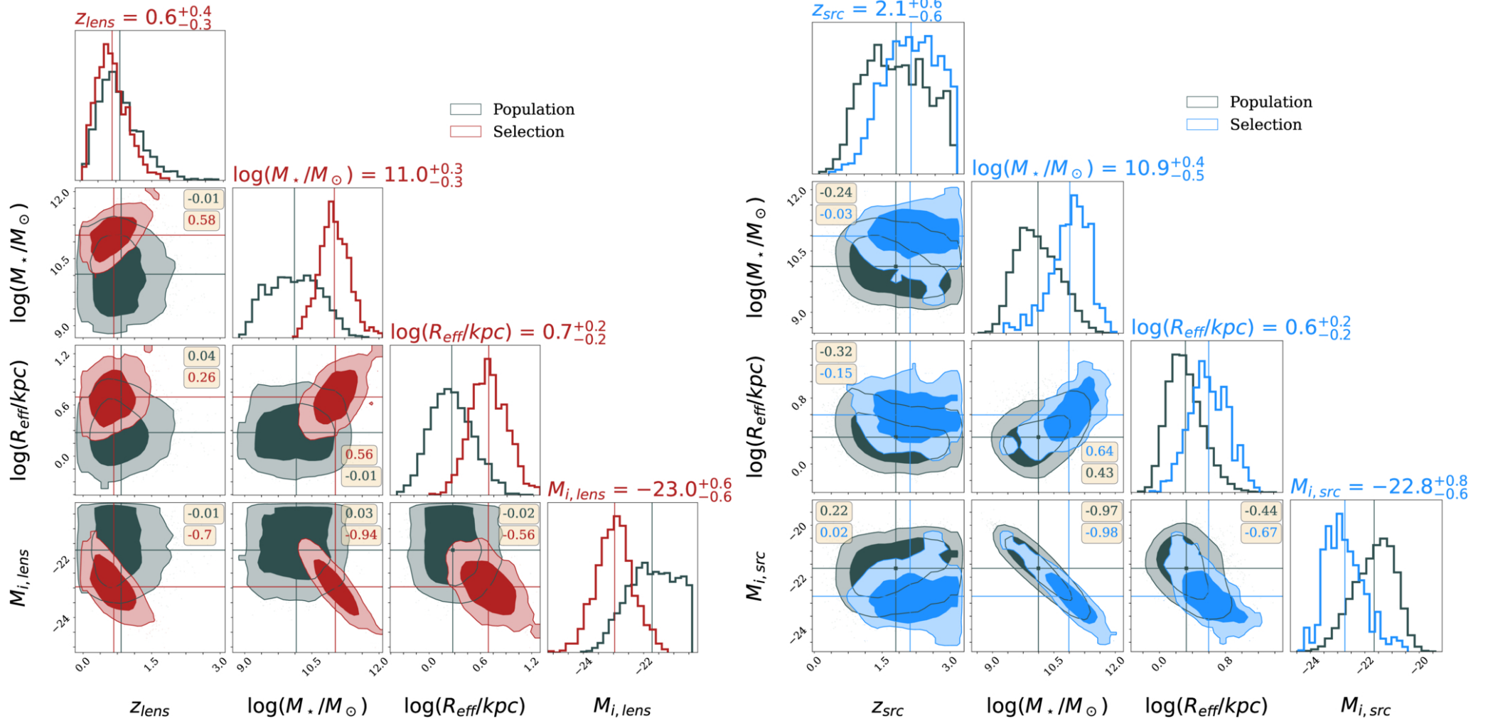
Figure 3. from Padmavathi Venkatraman et al 2026 Astron. J. 172 doi:10.3847/1538-3881/ae9e2b https://dx.doi.org/10.3847/1538-3881/ae9e2b © 2026. The Author(s). Published by the American Astronomical Society.
