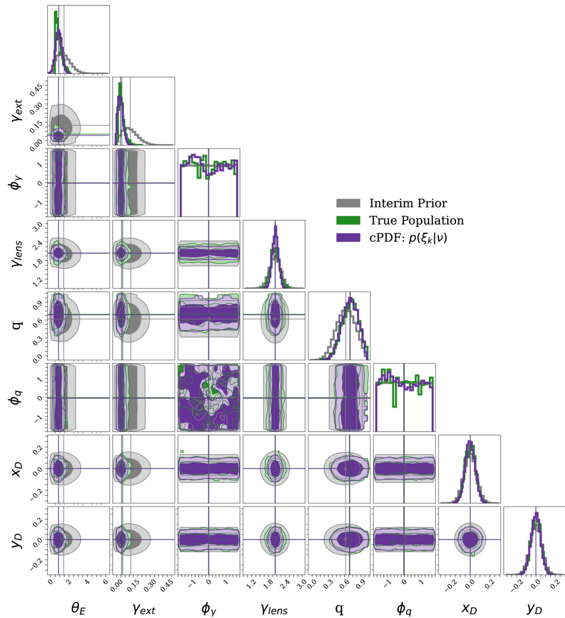
Figure 10. from Padmavathi Venkatraman et al 2026 Astron. J. 172 doi:10.3847/1538-3881/ae9e2b https://dx.doi.org/10.3847/1538-3881/ae9e2b © 2026. The Author(s). Published by the American Astronomical Society.
