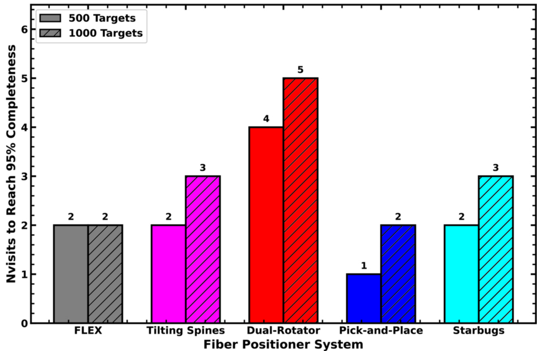
Figure 7. from Ummee T. Ahmed et al 2026 Astron. J. 172 doi:10.3847/1538-3881/ae9d7a https://dx.doi.org/10.3847/1538-3881/ae9d7a © 2026. The Author(s). Published by the American Astronomical Society.
