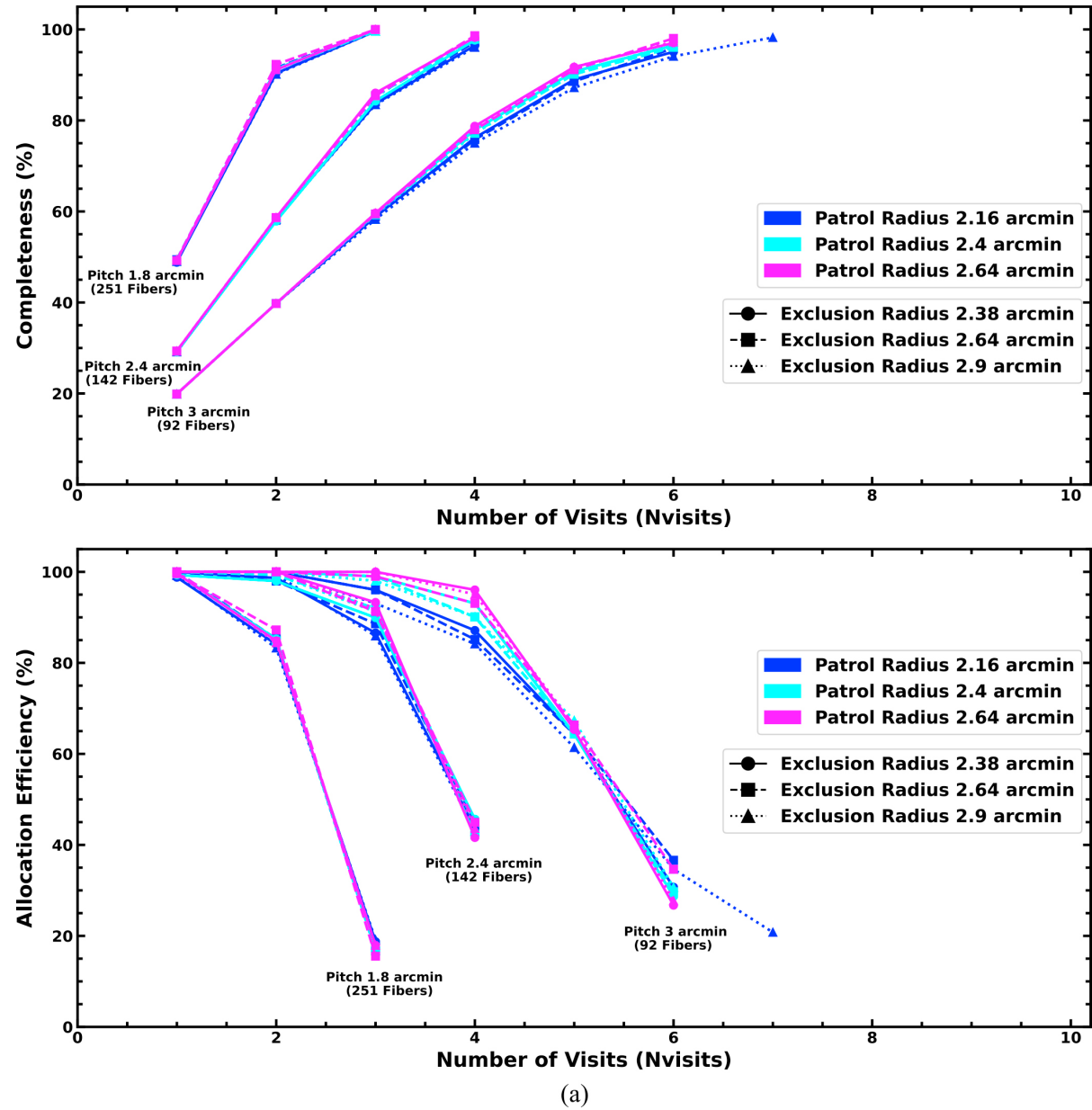
Figure 4. from Ummee T. Ahmed et al 2026 Astron. J. 172 doi:10.3847/1538-3881/ae9d7a https://dx.doi.org/10.3847/1538-3881/ae9d7a © 2026. The Author(s). Published by the American Astronomical Society.
