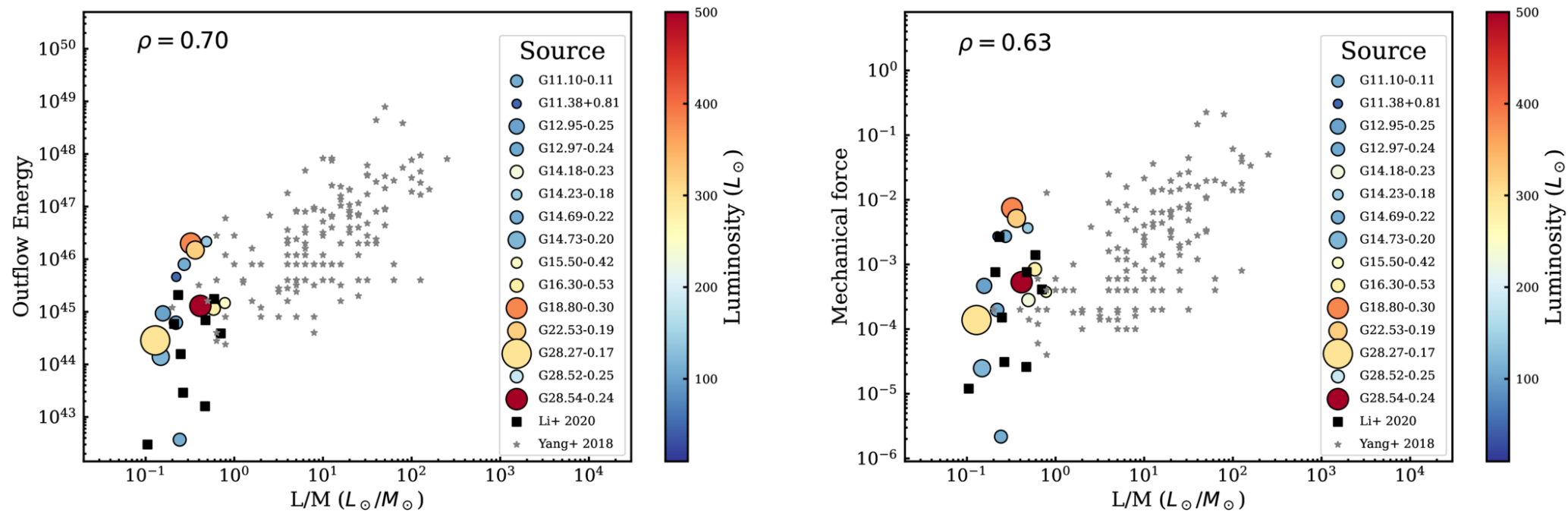
Figure 6. from Shuting Lin et al 2026 Astron. J. 172 doi:10.3847/1538-3881/ae9d5b https://dx.doi.org/10.3847/1538-3881/ae9d5b © 2026. The Author(s). Published by the American Astronomical Society.
