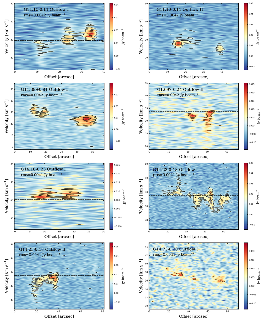
Figure 2. from Shuting Lin et al 2026 Astron. J. 172 doi:10.3847/1538-3881/ae9d5b https://dx.doi.org/10.3847/1538-3881/ae9d5b © 2026. The Author(s). Published by the American Astronomical Society.
