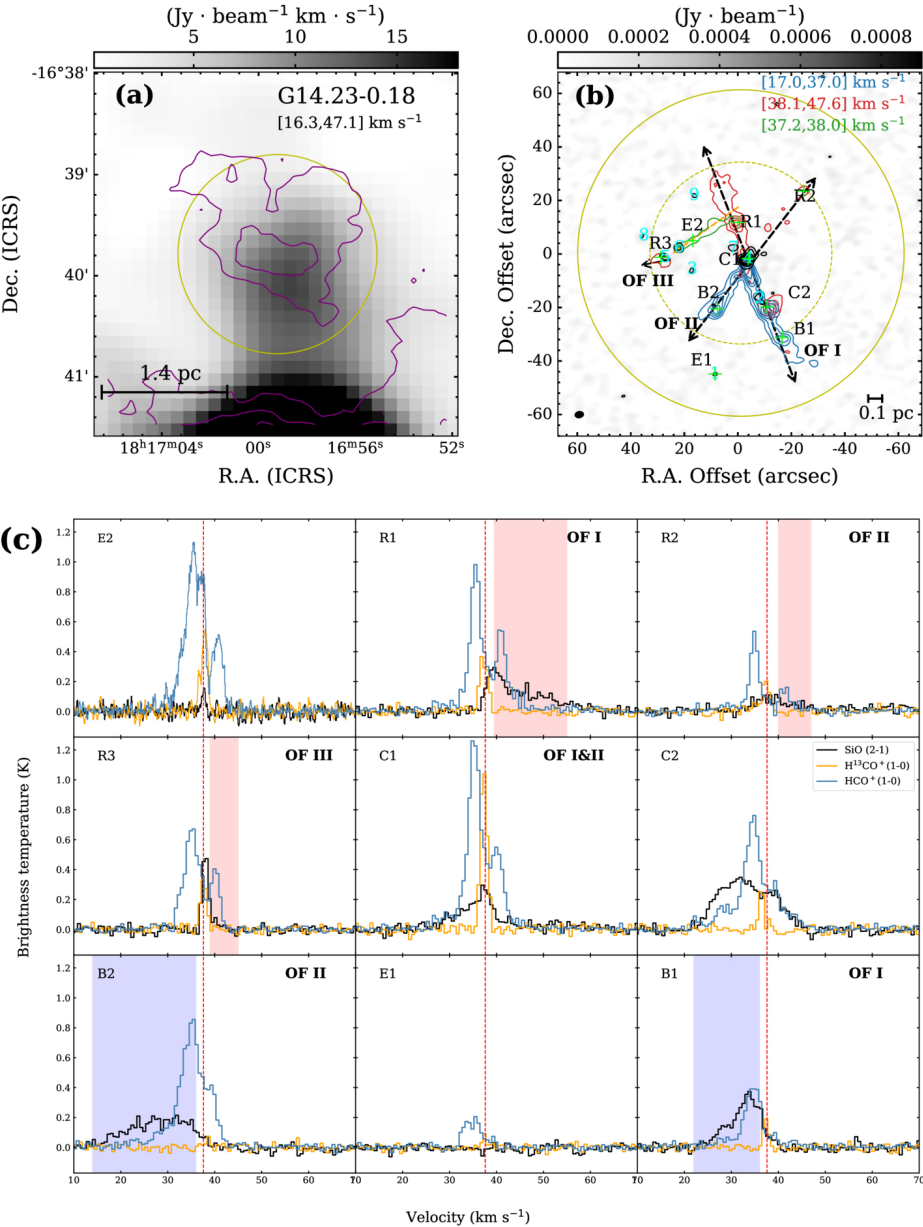
Figure 1. Integrated intensity maps and line profiles toward the observed sources. from Shuting Lin et al 2026 Astron. J. 172 doi:10.3847/1538-3881/ae9d5b https://dx.doi.org/10.3847/1538-3881/ae9d5b © 2026. The Author(s). Published by the American Astronomical Society.
