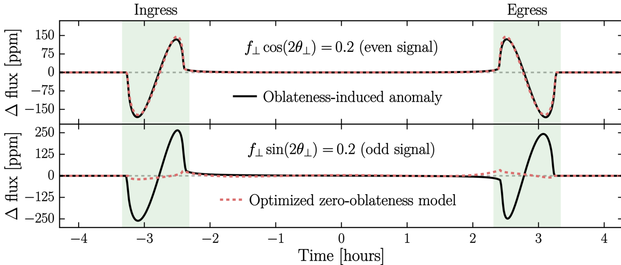
Figure 1. from Caleb Lammers and Joshua N. Winn 2026 Astron. J. 172 doi:10.3847/1538-3881/ae9d53 https://dx.doi.org/10.3847/1538-3881/ae9d53 © 2026. The Author(s). Published by the American Astronomical Society.
