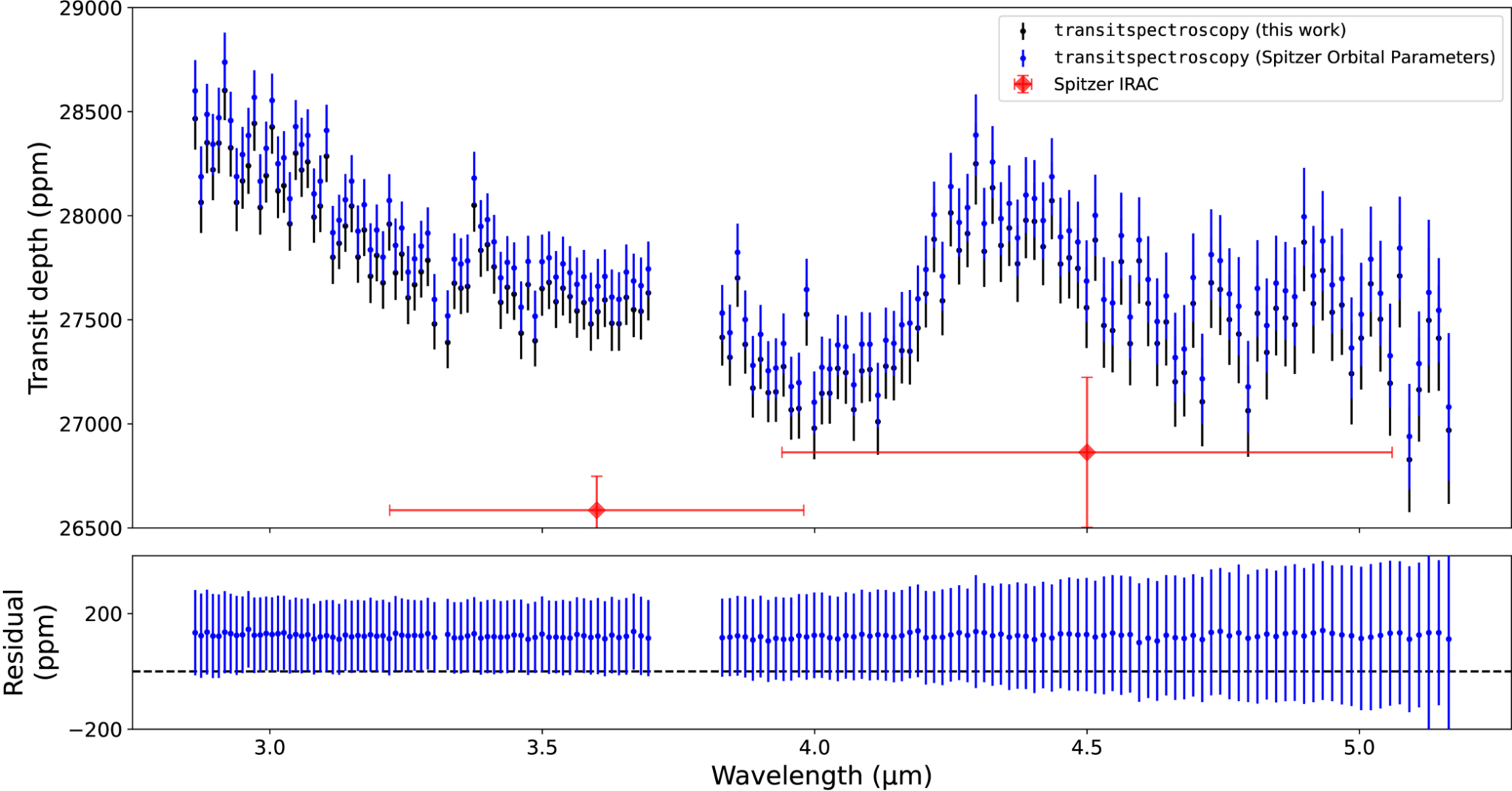
Figure B1. from Yanbo Pan et al 2026 Astron. J. 172 doi:10.3847/1538-3881/ae9cbc https://dx.doi.org/10.3847/1538-3881/ae9cbc © 2026. The Author(s). Published by the American Astronomical Society.
