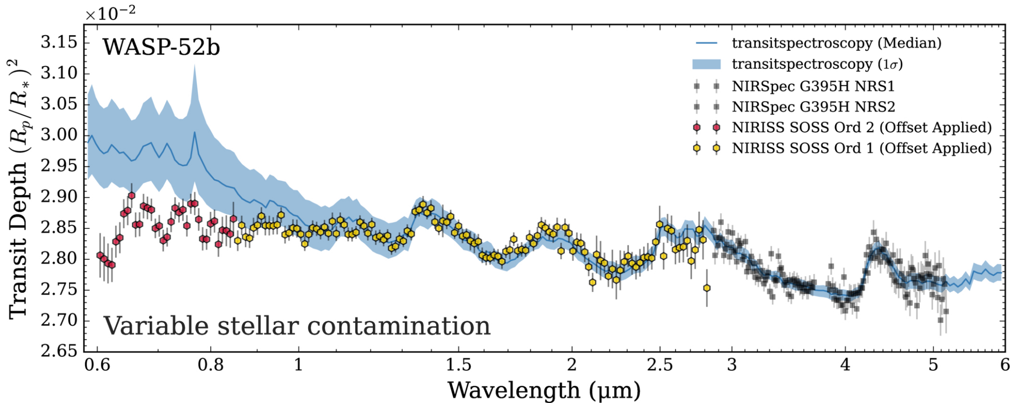
Figure 6. from Yanbo Pan et al 2026 Astron. J. 172 doi:10.3847/1538-3881/ae9cbc https://dx.doi.org/10.3847/1538-3881/ae9cbc © 2026. The Author(s). Published by the American Astronomical Society.
