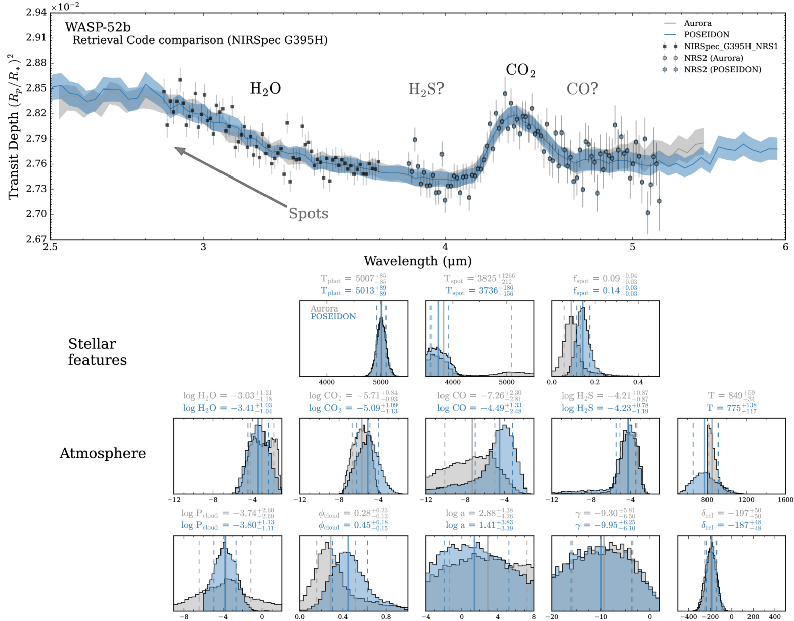
Figure 5. from Yanbo Pan et al 2026 Astron. J. 172 doi:10.3847/1538-3881/ae9cbc https://dx.doi.org/10.3847/1538-3881/ae9cbc © 2026. The Author(s). Published by the American Astronomical Society.
