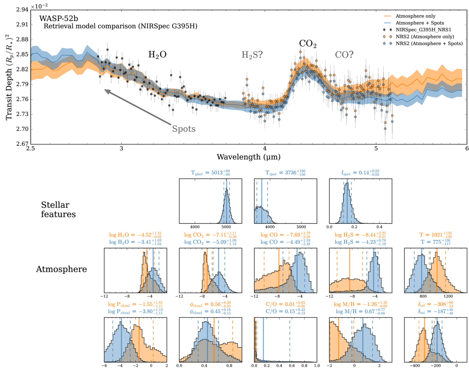
Figure 3. from Yanbo Pan et al 2026 Astron. J. 172 doi:10.3847/1538-3881/ae9cbc https://dx.doi.org/10.3847/1538-3881/ae9cbc © 2026. The Author(s). Published by the American Astronomical Society.
