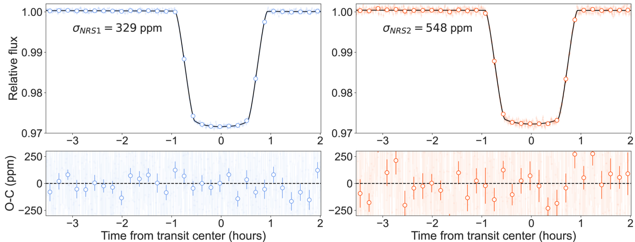
Figure 1. from Yanbo Pan et al 2026 Astron. J. 172 doi:10.3847/1538-3881/ae9cbc https://dx.doi.org/10.3847/1538-3881/ae9cbc © 2026. The Author(s). Published by the American Astronomical Society.
