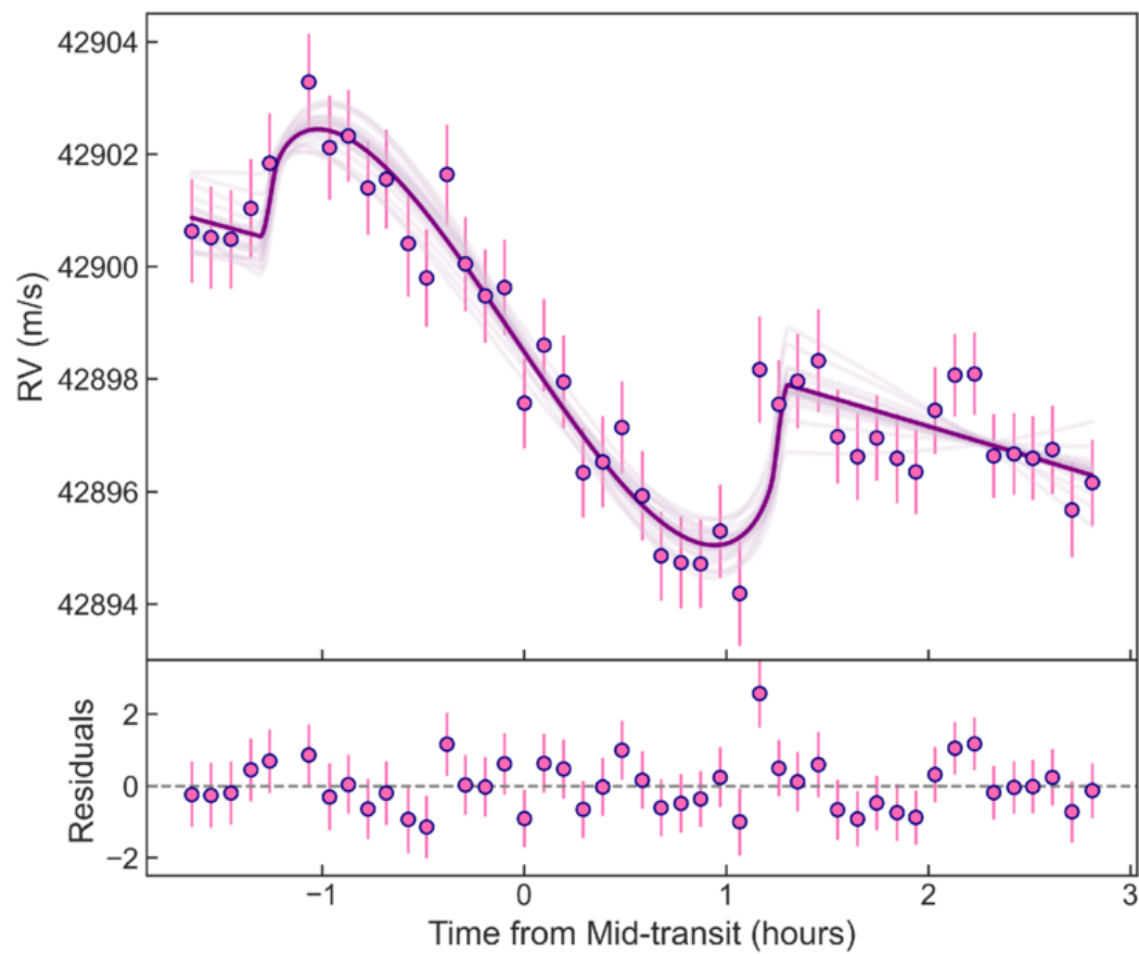
Figure 2. from Elina Y. Zhang et al 2026 Astron. J. 172 doi:10.3847/1538-3881/ae9c2b https://dx.doi.org/10.3847/1538-3881/ae9c2b © 2026. The Author(s). Published by the American Astronomical Society.
