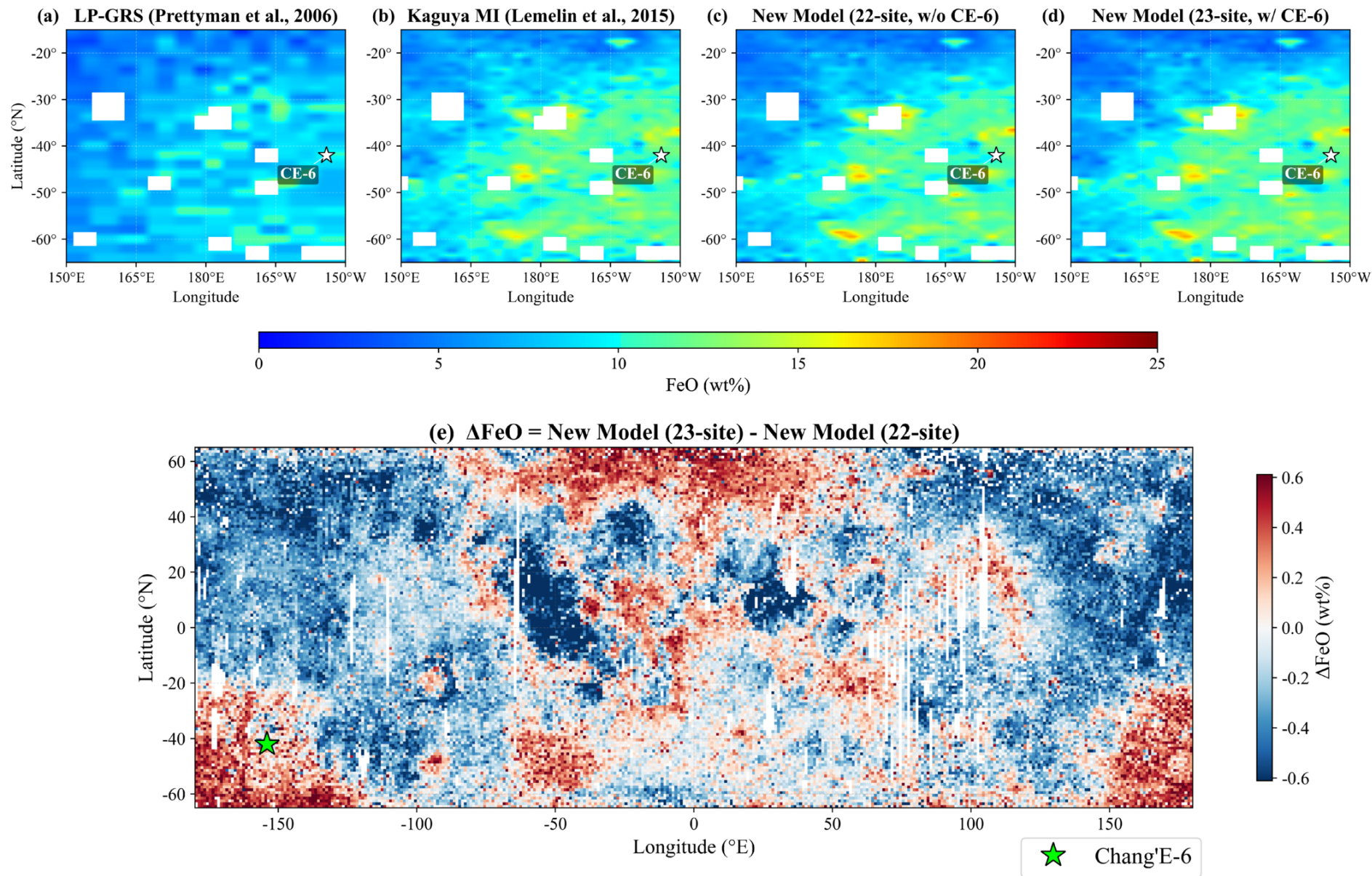
Figure 8. from Lijun Wang et al 2026 Astron. J. 172 doi:10.3847/1538-3881/ae9c28 https://dx.doi.org/10.3847/1538-3881/ae9c28 © 2026. The Author(s). Published by the American Astronomical Society.
