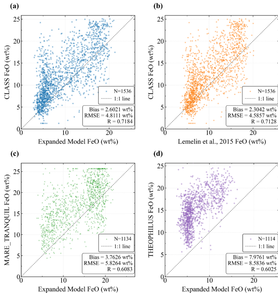
Figure 7. from Lijun Wang et al 2026 Astron. J. 172 doi:10.3847/1538-3881/ae9c28 https://dx.doi.org/10.3847/1538-3881/ae9c28 © 2026. The Author(s). Published by the American Astronomical Society.
