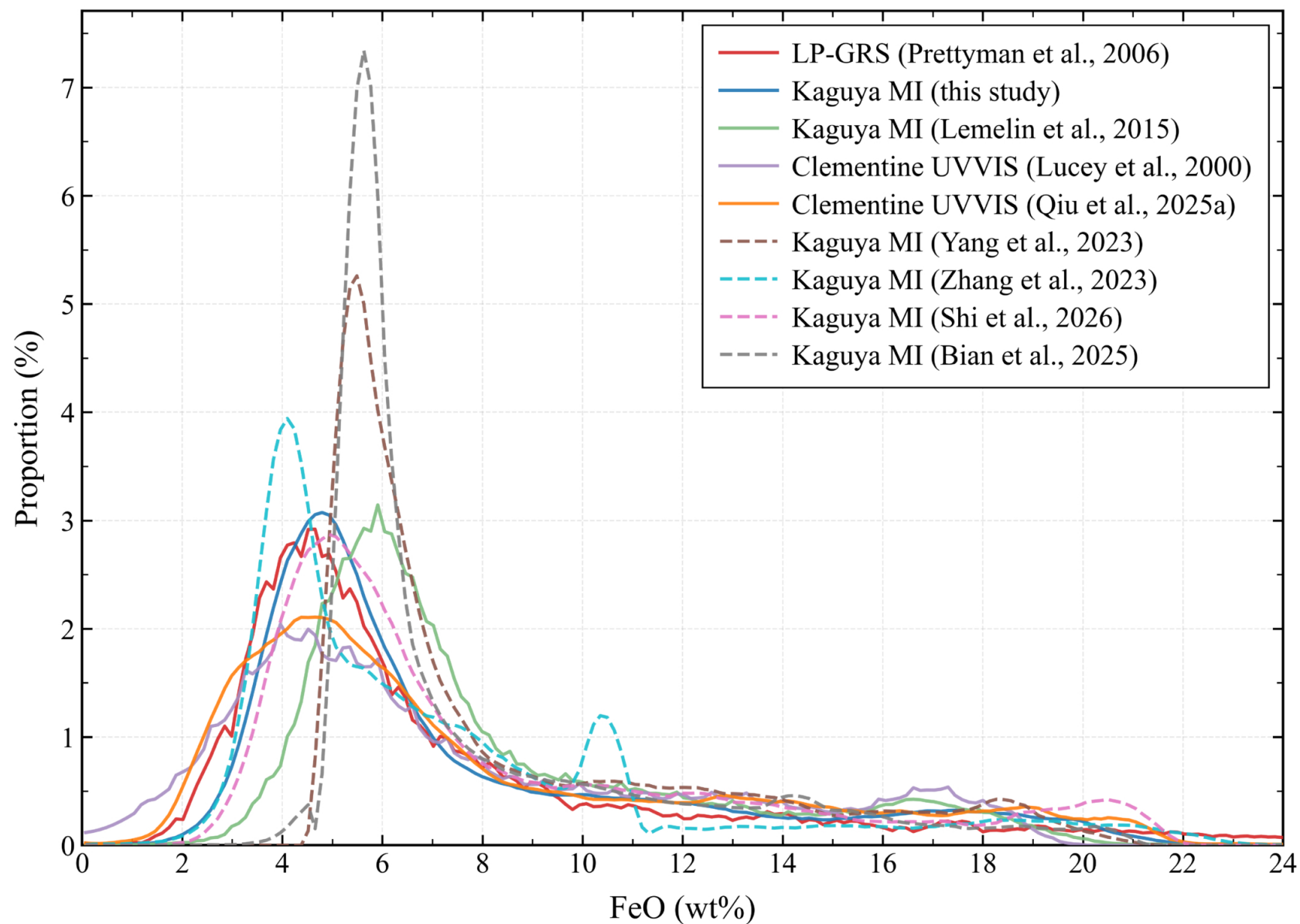
Figure 5. from Lijun Wang et al 2026 Astron. J. 172 doi:10.3847/1538-3881/ae9c28 https://dx.doi.org/10.3847/1538-3881/ae9c28 © 2026. The Author(s). Published by the American Astronomical Society.
