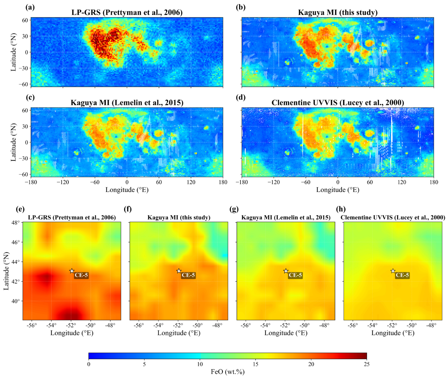
Figure 3. from Lijun Wang et al 2026 Astron. J. 172 doi:10.3847/1538-3881/ae9c28 https://dx.doi.org/10.3847/1538-3881/ae9c28 © 2026. The Author(s). Published by the American Astronomical Society.
