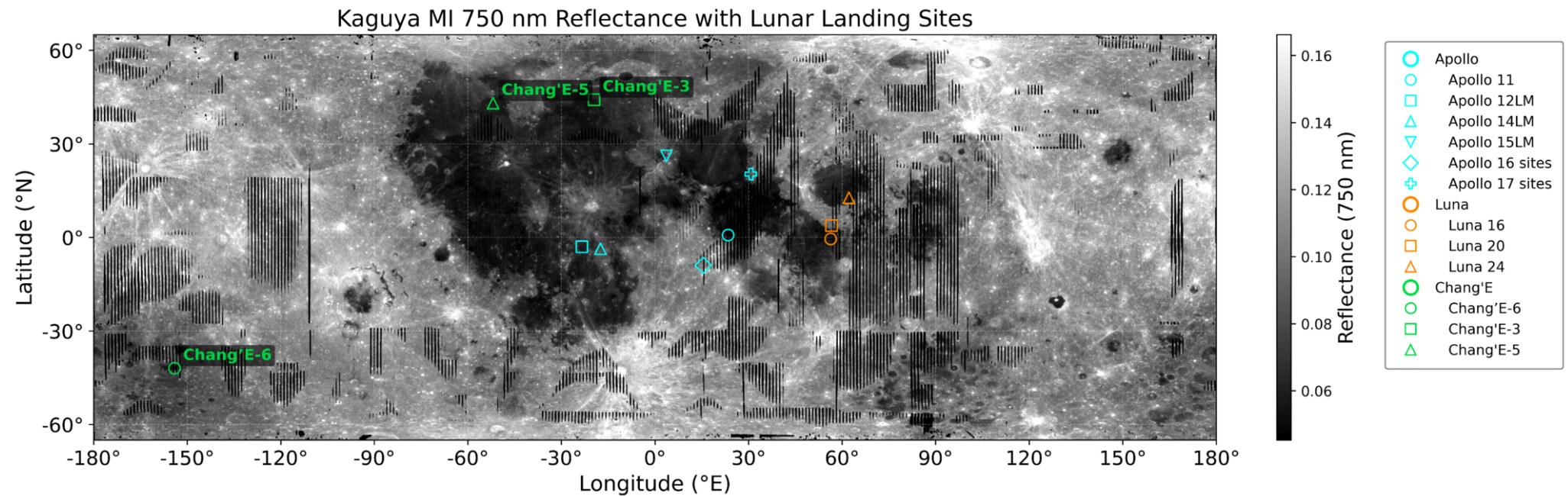
Figure 1. from Lijun Wang et al 2026 Astron. J. 172 doi:10.3847/1538-3881/ae9c28 https://dx.doi.org/10.3847/1538-3881/ae9c28 © 2026. The Author(s). Published by the American Astronomical Society.
