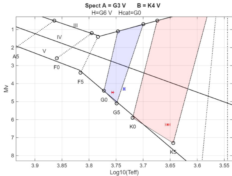
Figure 9. from Jack D. Drummond and Odell R. Reynolds 2026 Astron. J. 172 doi:10.3847/1538-3881/ae9bae https://dx.doi.org/10.3847/1538-3881/ae9bae © 2026. The Author(s). Published by the American Astronomical Society.
