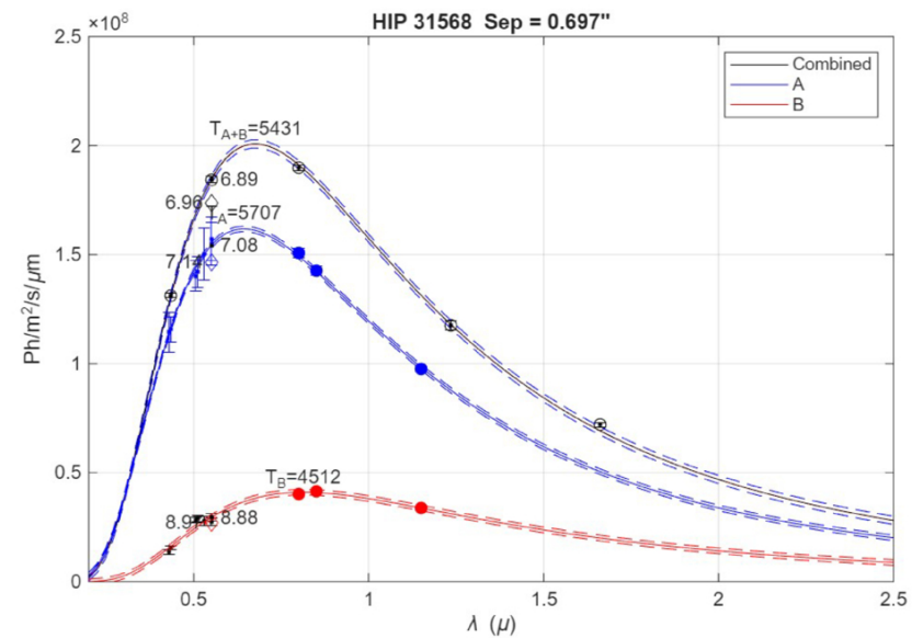
Figure 9. from Jack D. Drummond and Odell R. Reynolds 2026 Astron. J. 172 doi:10.3847/1538-3881/ae9bae https://dx.doi.org/10.3847/1538-3881/ae9bae © 2026. The Author(s). Published by the American Astronomical Society.
