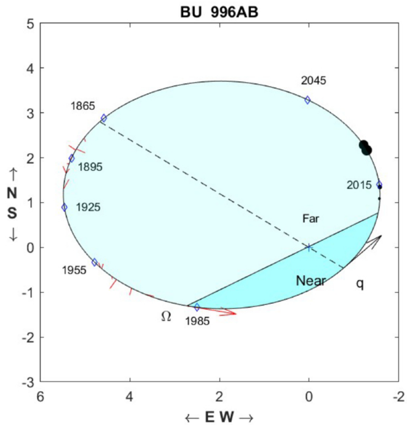
Figure 7. from Jack D. Drummond and Odell R. Reynolds 2026 Astron. J. 172 doi:10.3847/1538-3881/ae9bae https://dx.doi.org/10.3847/1538-3881/ae9bae © 2026. The Author(s). Published by the American Astronomical Society.
