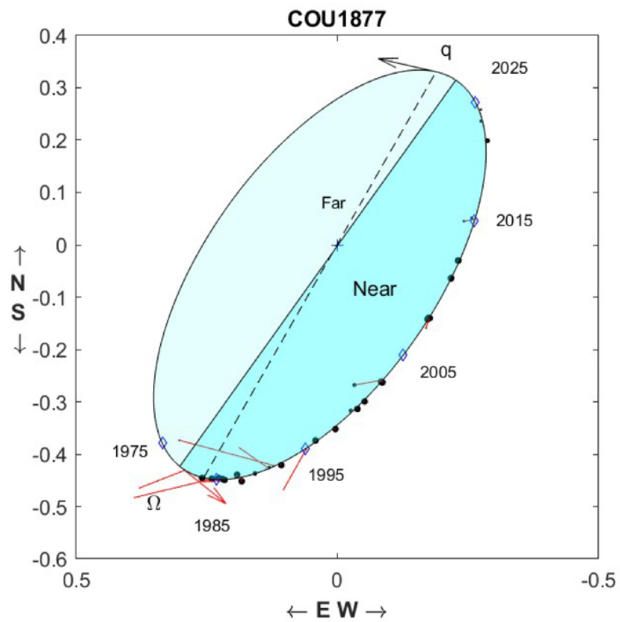
Figure 6. from Jack D. Drummond and Odell R. Reynolds 2026 Astron. J. 172 doi:10.3847/1538-3881/ae9bae https://dx.doi.org/10.3847/1538-3881/ae9bae © 2026. The Author(s). Published by the American Astronomical Society.
