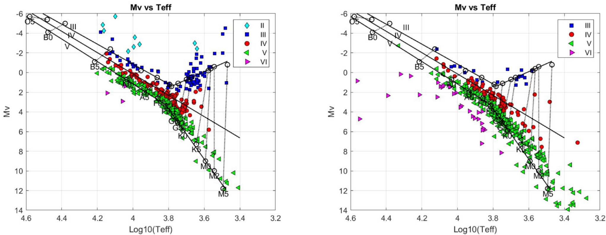
Figure 10. from Jack D. Drummond and Odell R. Reynolds 2026 Astron. J. 172 doi:10.3847/1538-3881/ae9bae https://dx.doi.org/10.3847/1538-3881/ae9bae © 2026. The Author(s). Published by the American Astronomical Society.
