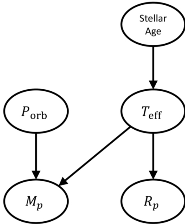
Figure 5. from Zehao Jin et al 2026 Astron. J. 172 doi:10.3847/1538-3881/ae9bab https://dx.doi.org/10.3847/1538-3881/ae9bab © 2026. The Author(s). Published by the American Astronomical Society.
