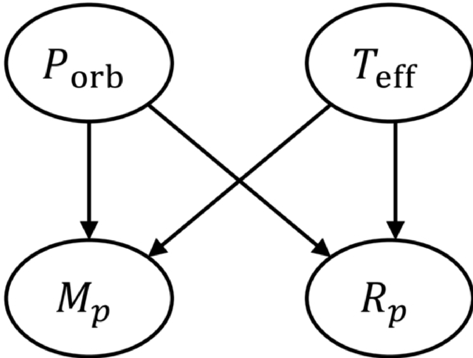
Figure 4. from Zehao Jin et al 2026 Astron. J. 172 doi:10.3847/1538-3881/ae9bab https://dx.doi.org/10.3847/1538-3881/ae9bab © 2026. The Author(s). Published by the American Astronomical Society.
