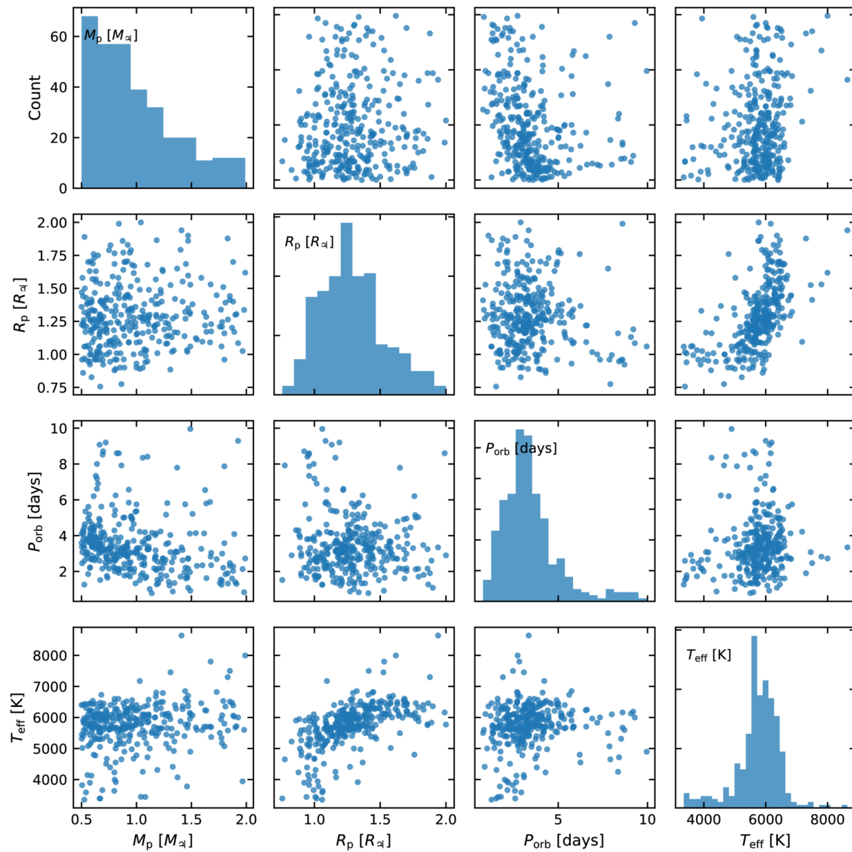
Figure 1. from Zehao Jin et al 2026 Astron. J. 172 doi:10.3847/1538-3881/ae9bab https://dx.doi.org/10.3847/1538-3881/ae9bab © 2026. The Author(s). Published by the American Astronomical Society.
