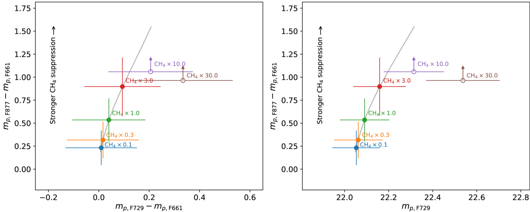
Figure 7. from Yiming Zhu et al 2026 Astron. J. 172 doi:10.3847/1538-3881/ae9b04 https://dx.doi.org/10.3847/1538-3881/ae9b04 © 2026. The Author(s). Published by the American Astronomical Society.
