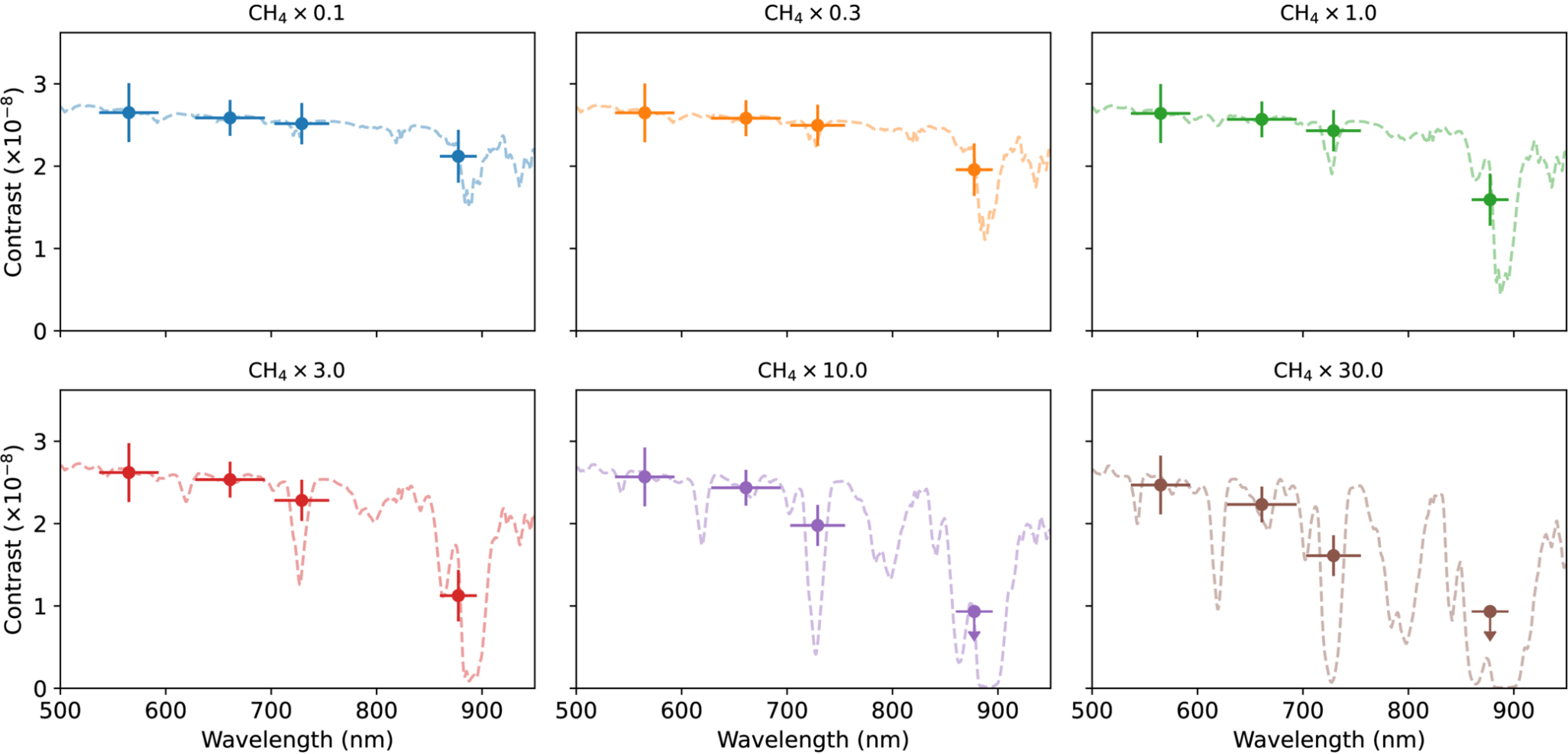
Figure 6. from Yiming Zhu et al 2026 Astron. J. 172 doi:10.3847/1538-3881/ae9b04 https://dx.doi.org/10.3847/1538-3881/ae9b04 © 2026. The Author(s). Published by the American Astronomical Society.
