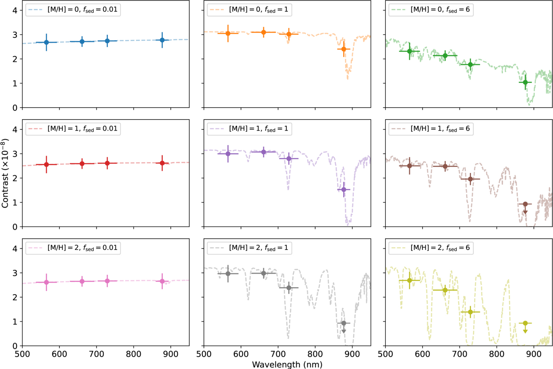
Figure 5. from Yiming Zhu et al 2026 Astron. J. 172 doi:10.3847/1538-3881/ae9b04 https://dx.doi.org/10.3847/1538-3881/ae9b04 © 2026. The Author(s). Published by the American Astronomical Society.
