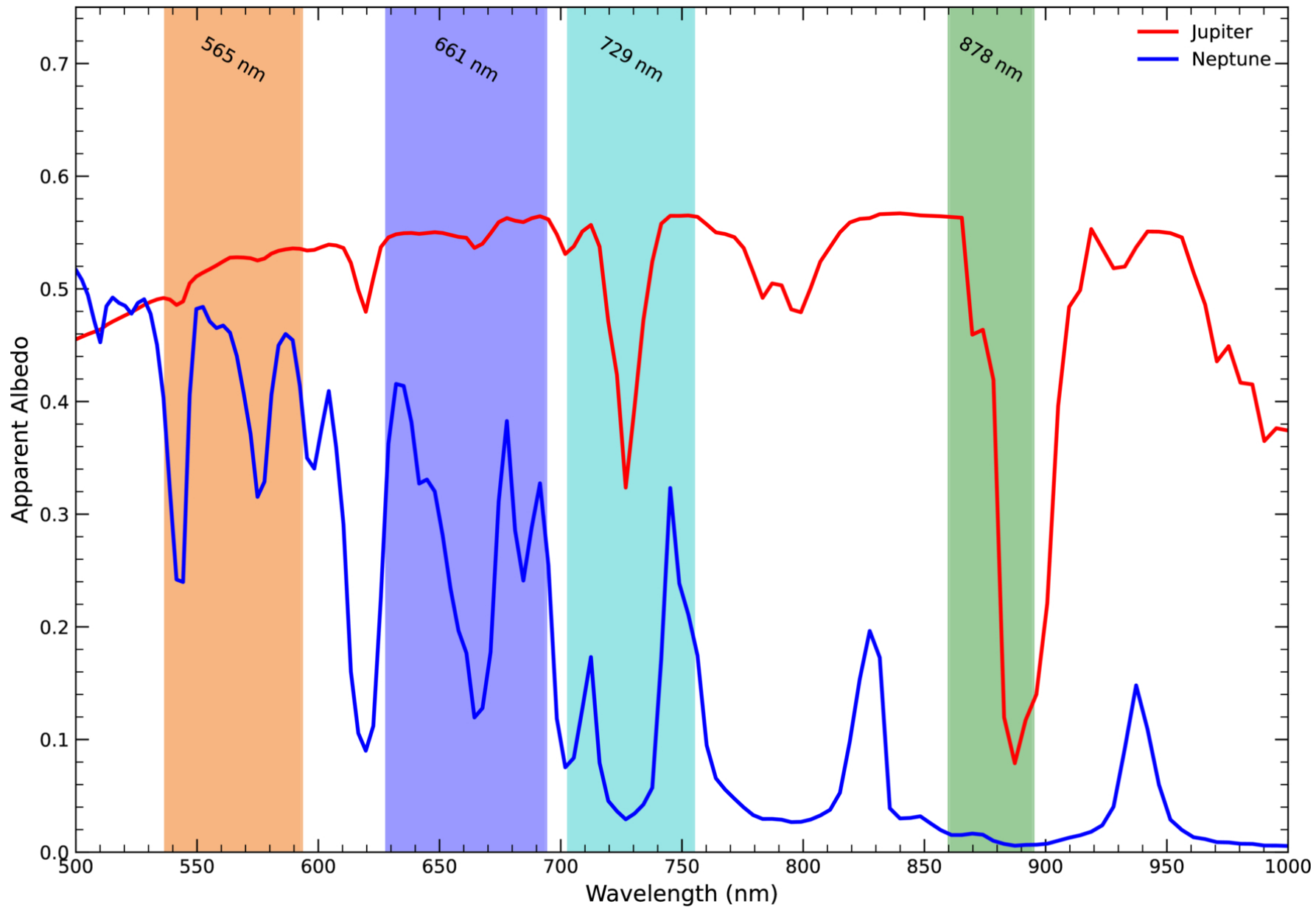
Figure 3. from Yiming Zhu et al 2026 Astron. J. 172 doi:10.3847/1538-3881/ae9b04 https://dx.doi.org/10.3847/1538-3881/ae9b04 © 2026. The Author(s). Published by the American Astronomical Society.
