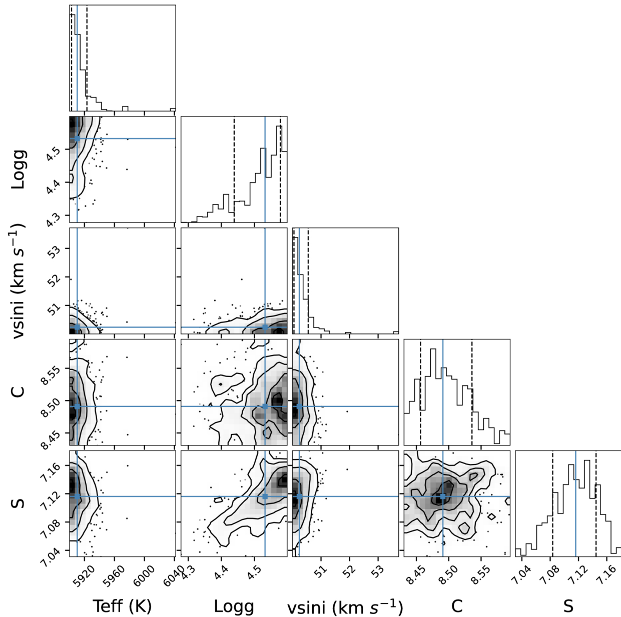
Figure 2. from Aneesh Baburaj et al 2026 Astron. J. 172 doi:10.3847/1538-3881/ae9afe https://dx.doi.org/10.3847/1538-3881/ae9afe © 2026. The Author(s). Published by the American Astronomical Society.
