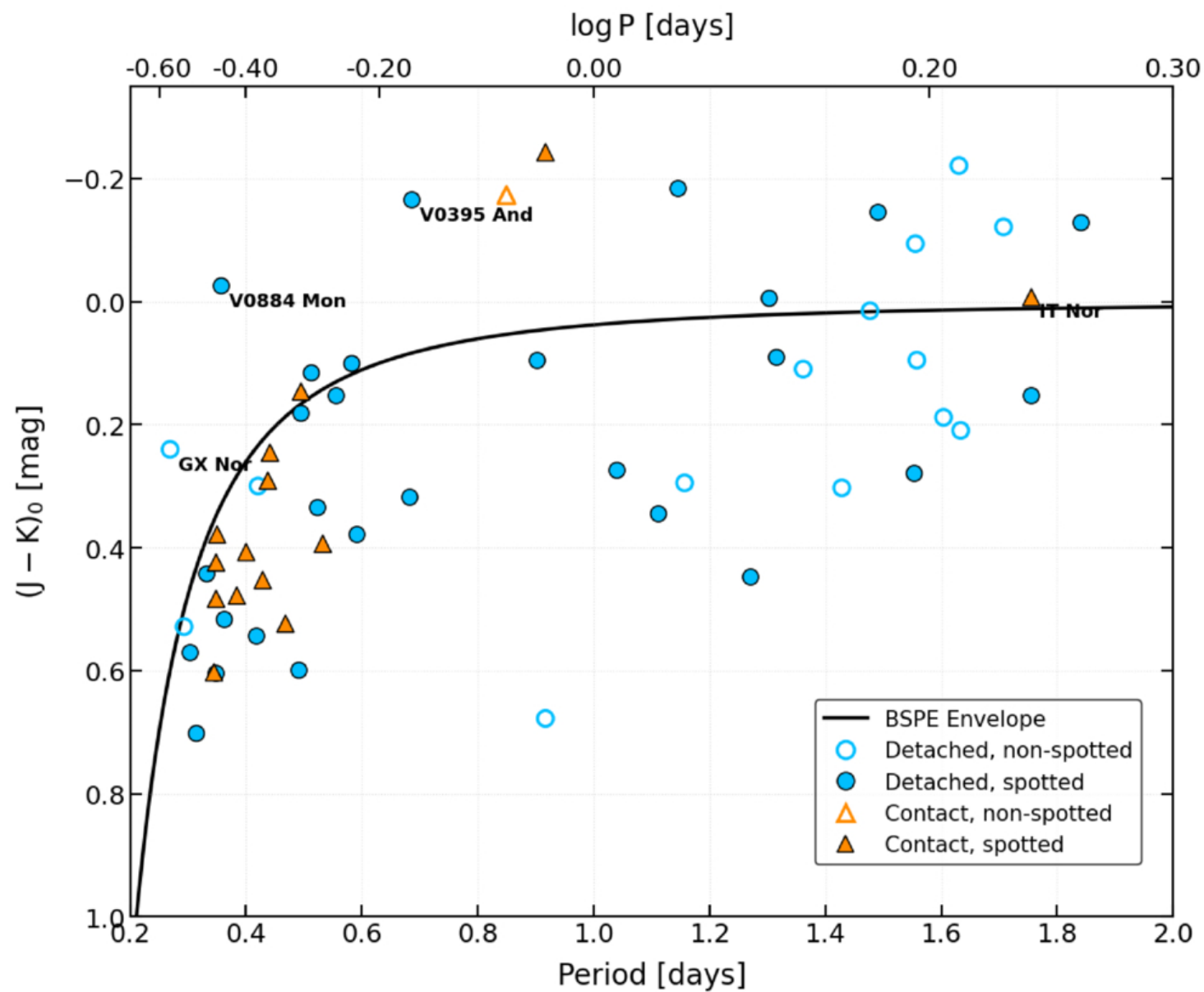
Figure 2. from Martin Vako et al 2026 Astron. J. 172 doi:10.3847/1538-3881/ae9a7b https://dx.doi.org/10.3847/1538-3881/ae9a7b © 2026. The Author(s). Published by the American Astronomical Society.
