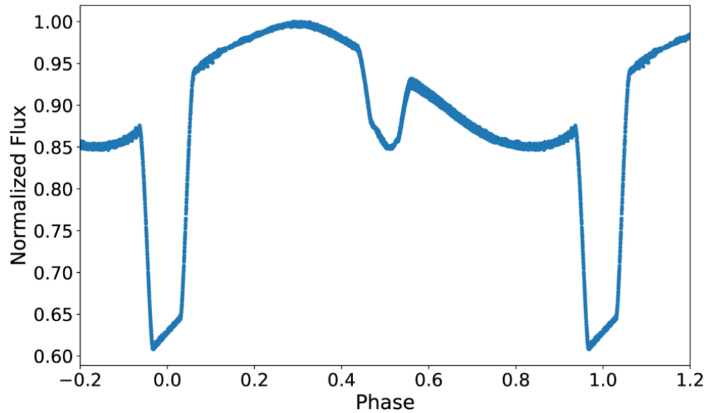
Figure 1. from Martin Vako et al 2026 Astron. J. 172 doi:10.3847/1538-3881/ae9a7b https://dx.doi.org/10.3847/1538-3881/ae9a7b © 2026. The Author(s). Published by the American Astronomical Society.
