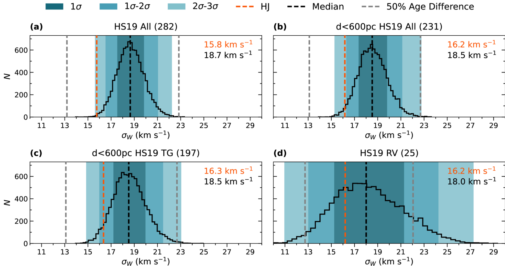
Figure 3. from Qingru Hu et al 2026 Astron. J. 172 doi:10.3847/1538-3881/ae9a77 https://dx.doi.org/10.3847/1538-3881/ae9a77 © 2026. The Author(s). Published by the American Astronomical Society.
