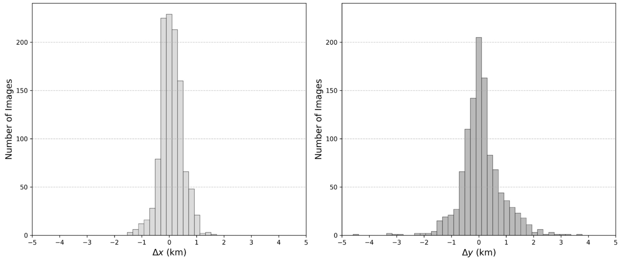
Figure 4. from Wangxin Lai et al 2026 Astron. J. 172 doi:10.3847/1538-3881/ae99da https://dx.doi.org/10.3847/1538-3881/ae99da © 2026. The Author(s). Published by the American Astronomical Society.
