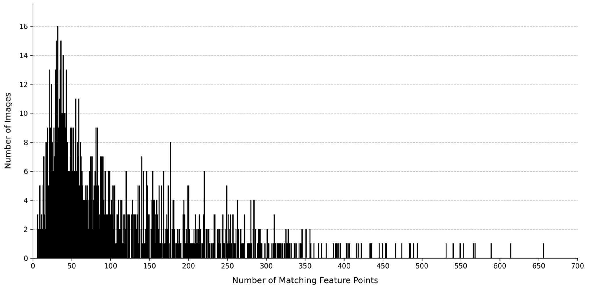
Figure 3. from Wangxin Lai et al 2026 Astron. J. 172 doi:10.3847/1538-3881/ae99da https://dx.doi.org/10.3847/1538-3881/ae99da © 2026. The Author(s). Published by the American Astronomical Society.
