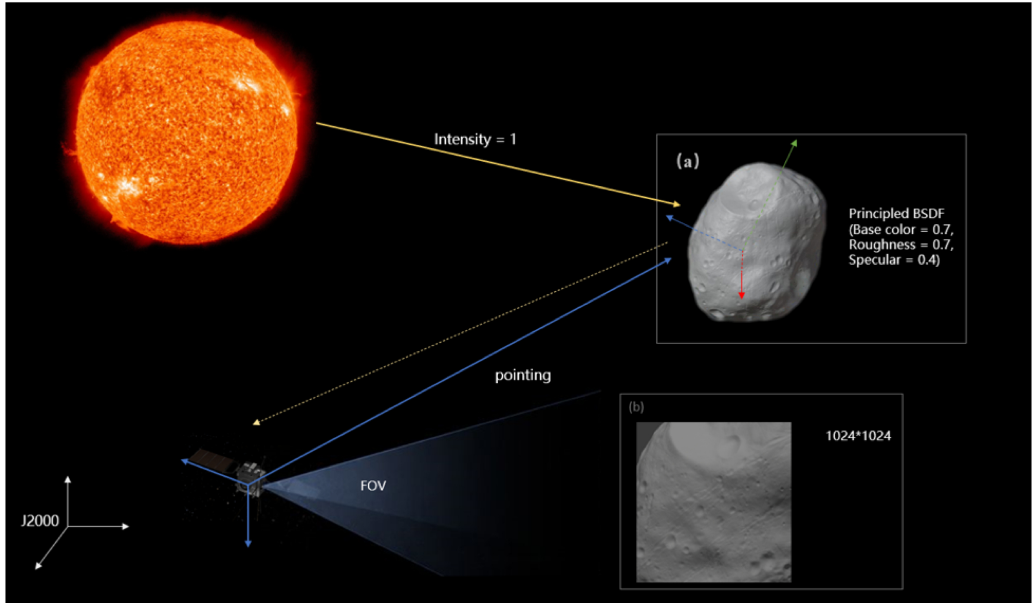
Figure 1. from Wangxin Lai et al 2026 Astron. J. 172 doi:10.3847/1538-3881/ae99da https://dx.doi.org/10.3847/1538-3881/ae99da © 2026. The Author(s). Published by the American Astronomical Society.
