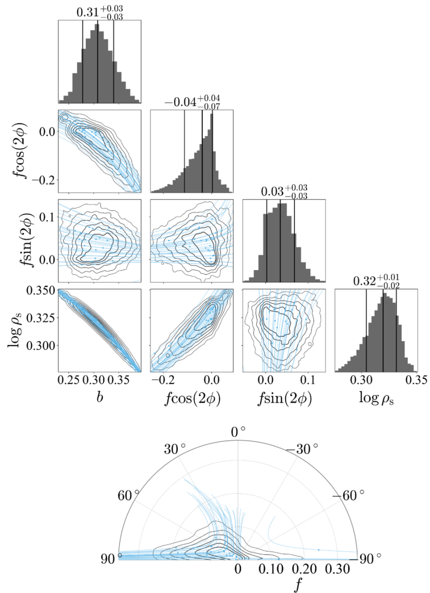
Figure 7. from Shotaro Tada 2026 Astron. J. 172 doi:10.3847/1538-3881/ae9947 https://dx.doi.org/10.3847/1538-3881/ae9947 © 2026. The Author(s). Published by the American Astronomical Society.
