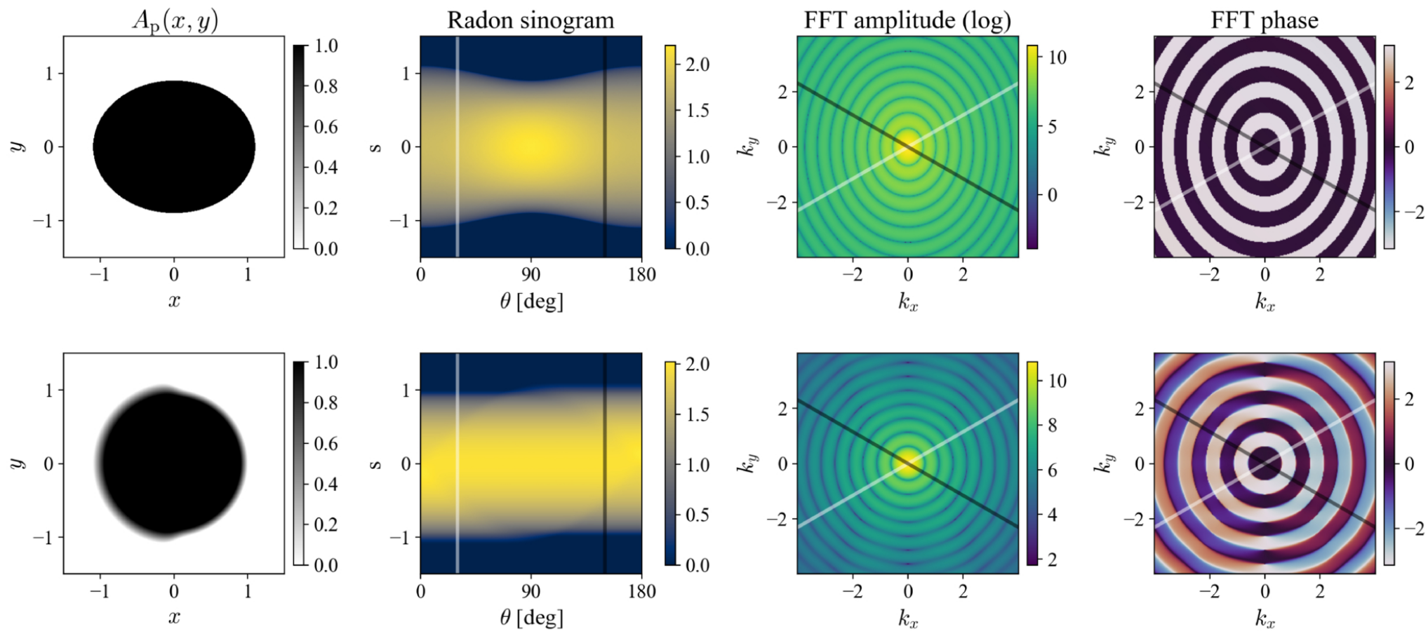
Figure 4. from Shotaro Tada 2026 Astron. J. 172 doi:10.3847/1538-3881/ae9947 https://dx.doi.org/10.3847/1538-3881/ae9947 © 2026. The Author(s). Published by the American Astronomical Society.
