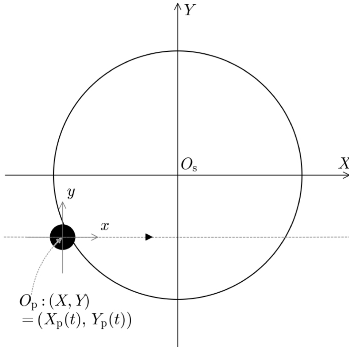
Figure 1. from Shotaro Tada 2026 Astron. J. 172 doi:10.3847/1538-3881/ae9947 https://dx.doi.org/10.3847/1538-3881/ae9947 © 2026. The Author(s). Published by the American Astronomical Society.
