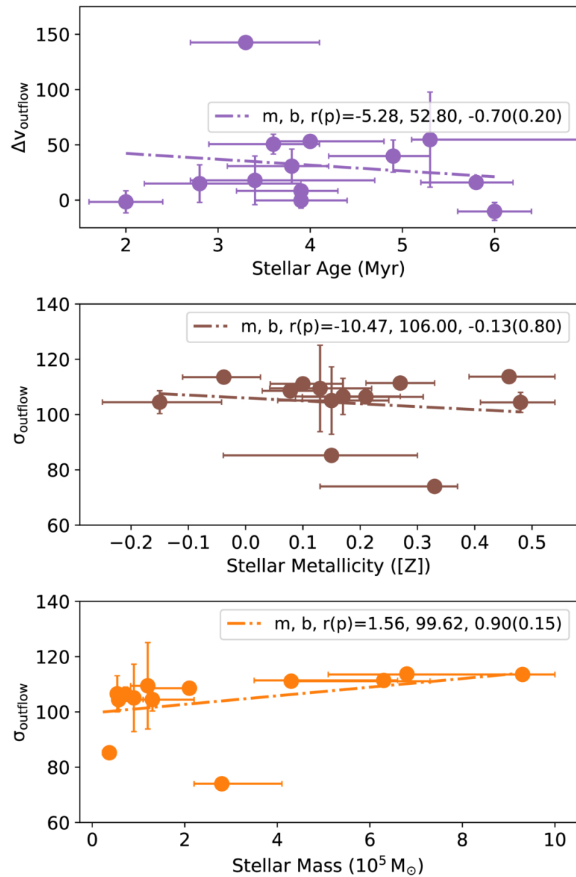
Figure 9. from Adarsh Ranjan et al 2026 Astron. J. 172 doi:10.3847/1538-3881/ae9943 https://dx.doi.org/10.3847/1538-3881/ae9943 © 2026. The Author(s). Published by the American Astronomical Society.
