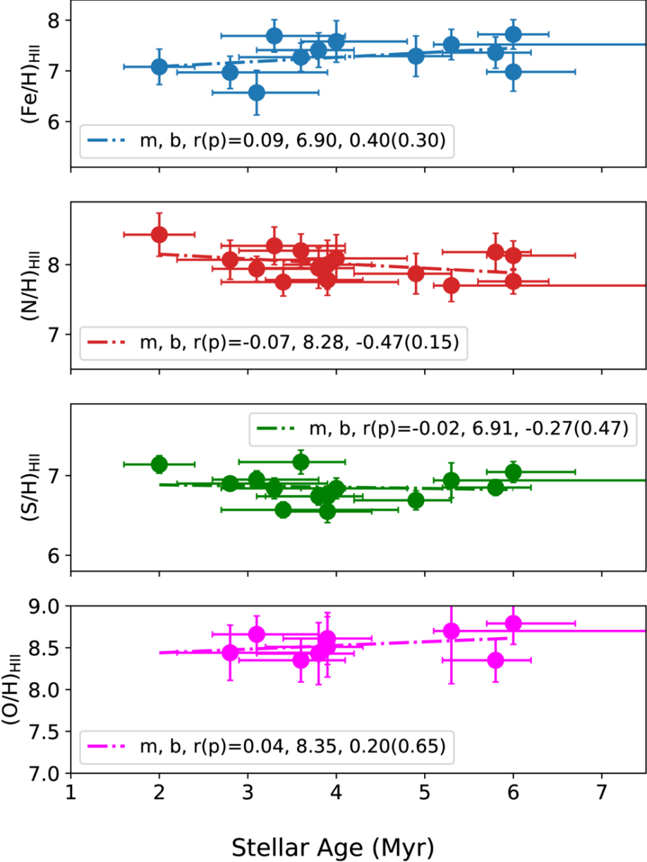
Figure 8. from Adarsh Ranjan et al 2026 Astron. J. 172 doi:10.3847/1538-3881/ae9943 https://dx.doi.org/10.3847/1538-3881/ae9943 © 2026. The Author(s). Published by the American Astronomical Society.
