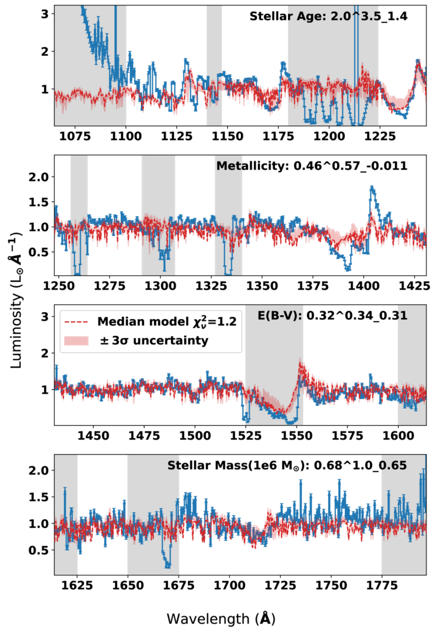
Figure F2. from Adarsh Ranjan et al 2026 Astron. J. 172 doi:10.3847/1538-3881/ae9943 https://dx.doi.org/10.3847/1538-3881/ae9943 © 2026. The Author(s). Published by the American Astronomical Society.
